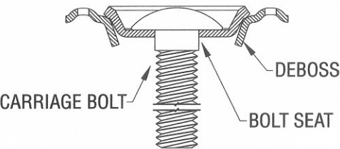
TYPICAL INSTALLATION
