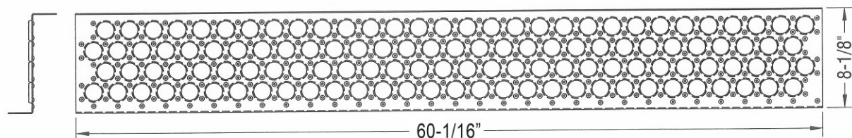
“A” END - END PLATFORM
