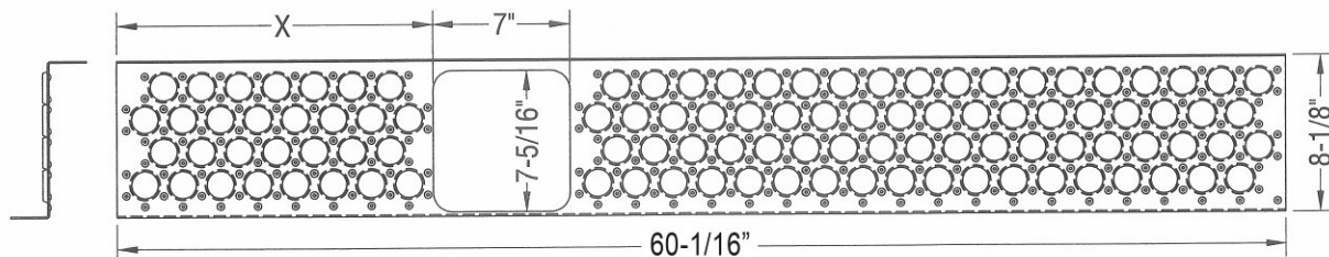
“B” END, CLOSED BACK END PLATFORM *Special Order
