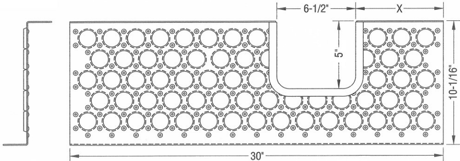
OPEN BACK BRAKE STEP WITH COLLAR
