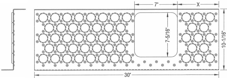
CLOSED BACK BRAKE STEP *Special Order
