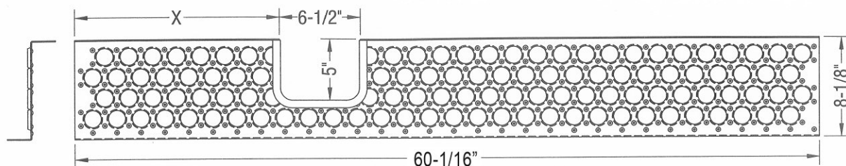
“B” END, OPEN BACK END PLATFORM WITH COLLAR
