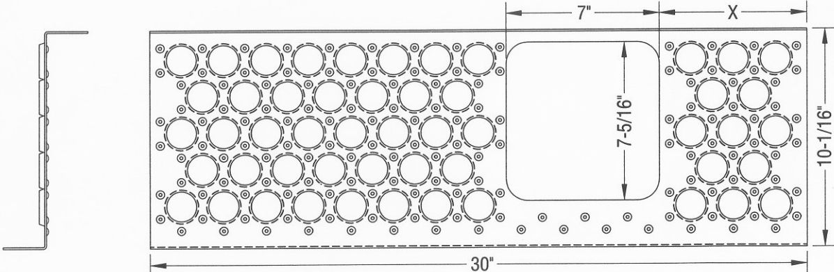
CLOSED BACK BRAKE STEP *Special Order
