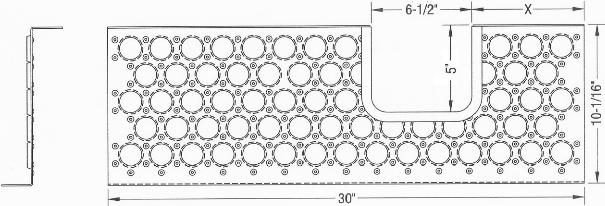
OPEN BACK BRAKE STEP WITH COLLAR
