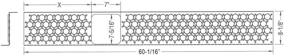
“B” END, CLOSED BACK END PLATFORM
