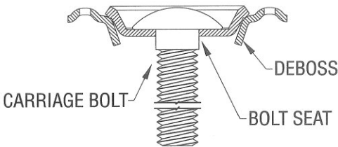
TYPICAL INSTALLATION
